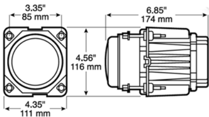
PM-710 Combo low and high beam
