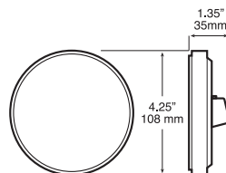
PM-1217A-9 light module
