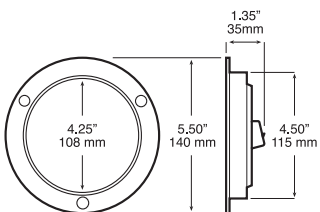
Flange mount
