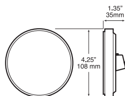
PM-1217F-9 light module
