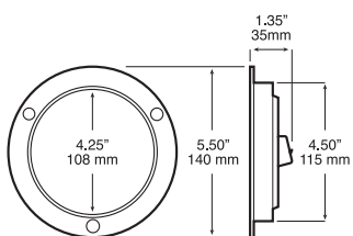
Flange mount
