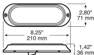
Surface mount with bracket
