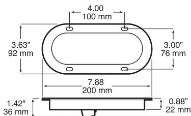
Flange mount
