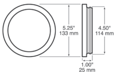
PM-1217G-R-426 flush mount
